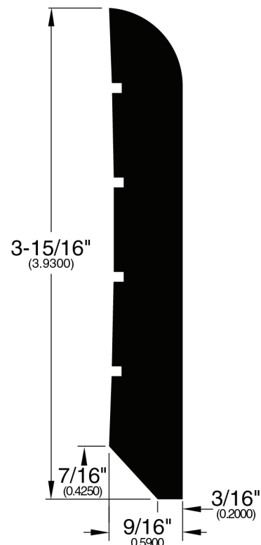
Wall Base (294)
