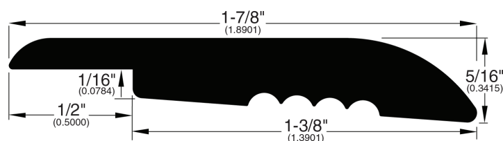
Overlap Reducer (297)
