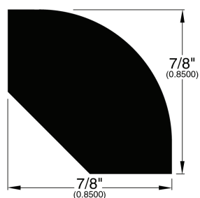
Quarter Round (296)
