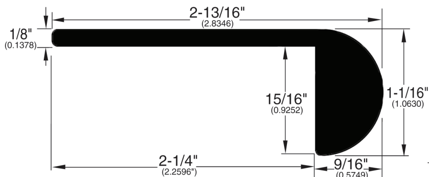
Stair Nose (298)
