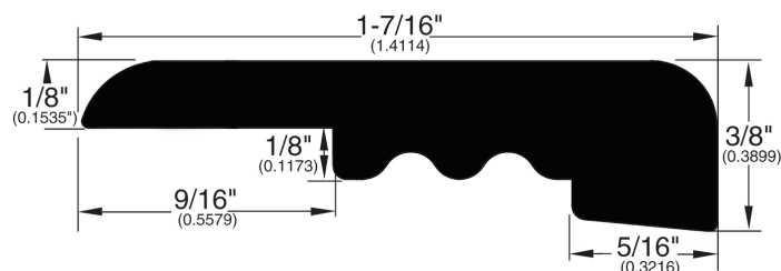
Square Nose (300)
